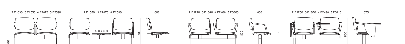
PANCA - BENCH
