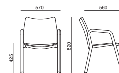
SEDIA - CHAIR
