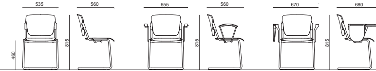
SLITTA - CANTILEVER CHAIR
